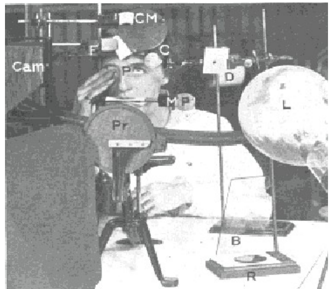
Fig. 24. Arrangements for Photographing Images Reflected From the Eyeball -- CM, concave mirror in which the subject may observe the images reflected from various parts of her eye- C, condenser; D, diaphragm; L, 1000-watt lamp; F, forehead rest; MP, bar which the subject grasps with her teeth for the purpose of holding her head steady- P, plane mirror upon which is pasted a letter of diamond type and in which is reflected a Snellen test card twenty feet behind the subject (the mirror is just above the letter P); CAM, camera; Pr, perimeter used to measure the angle of the light to the eye; R, plane mirror reflecting light from the 1000-watt lamp upon the eye, which otherwise would be in total darkness except for the part from which the highly condensed image of the filament is reflected; B, blue glass screen used to modify the light reflected from the mirror R. When the subject read the bottom line of the Snellen test card reflected in the mirror P her eye was at rest, and when she saw the letter of diamond type distinctly it was accommodated ten diopters, as demonstrated by the retinoscope.
